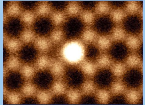
Si atom substituting for two C atoms in monolayer graphene: ADF image from Nion UltraSTEM™ at 60 keV. Courtesy W. Zhou and J.-C. Idrobo, ORNL
